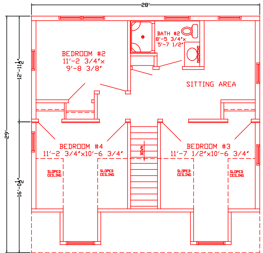
SECOND FLOOR
