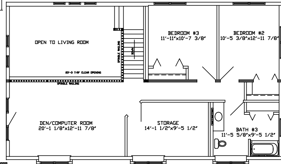
SECOND FLOOR
